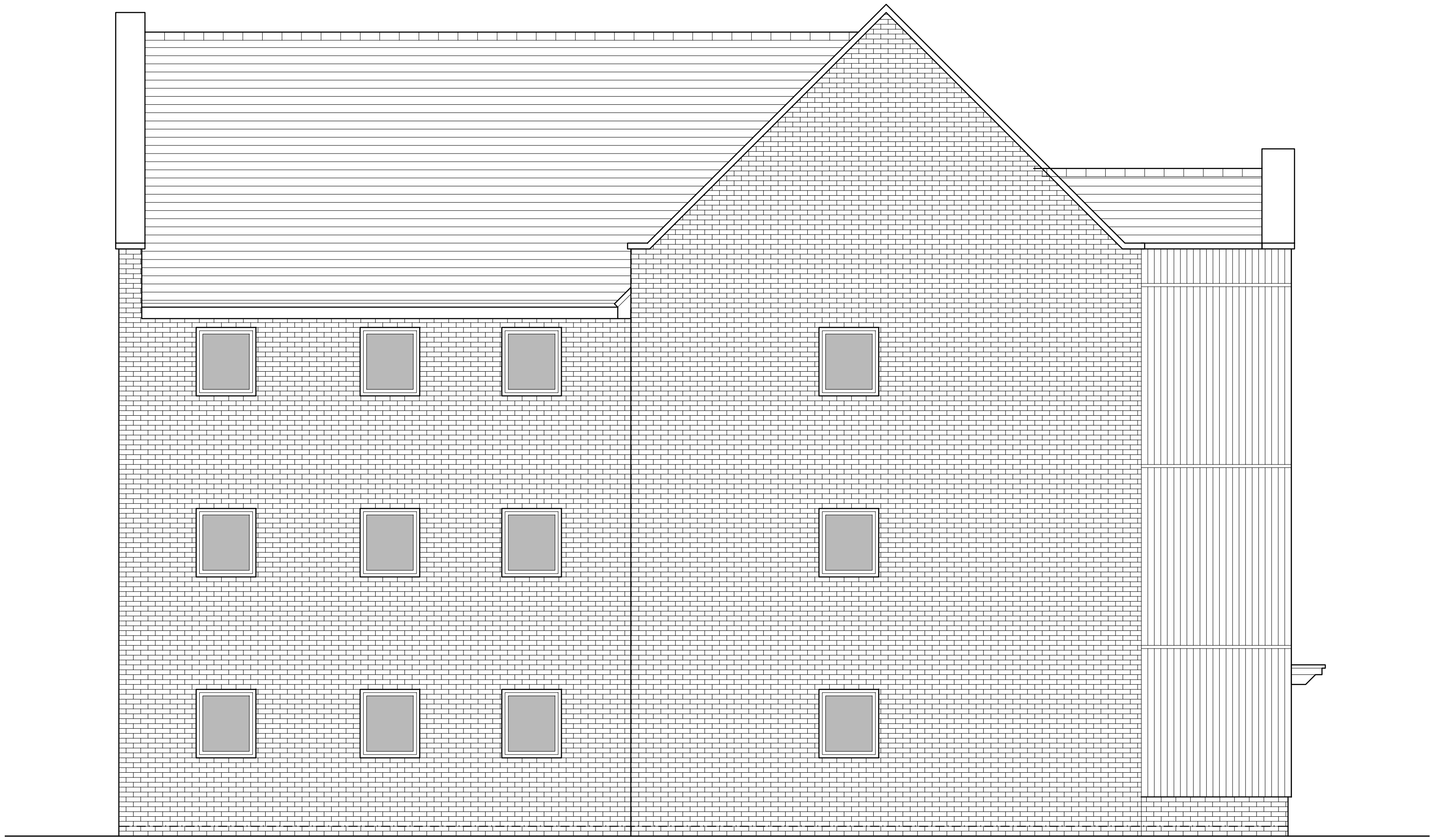
REAR ELEVATION
